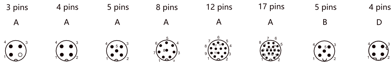
Contact Layouts/针孔排布(Front View/前视图)
