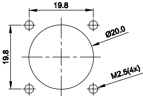
MOUNTING HOLE
