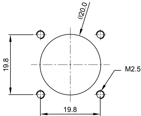
Mounting Holes
