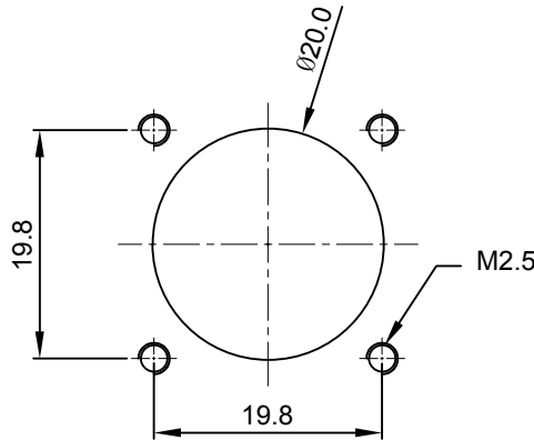
Mounting Holes
