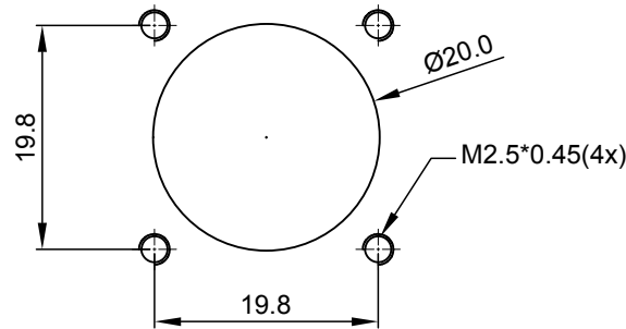
Mounting Holes
