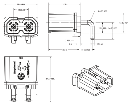
C10-747795-000 RADSOK® Receptacle, 3.6mm
