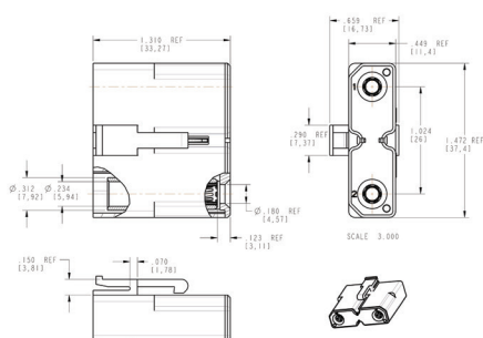
C10-752160-000 RADSOK® Plug, 1500V
