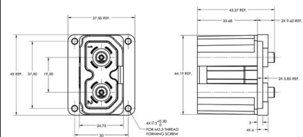
C10-752163-000 RADSOK® Receptacle, 5.7mm
