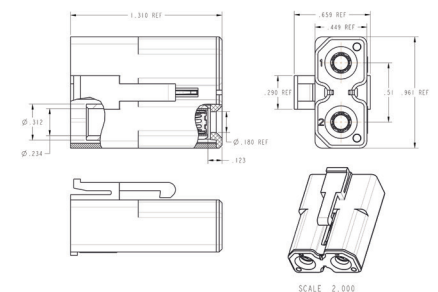
C10-752158-000 RADSOK® Plug, 3.6mm
