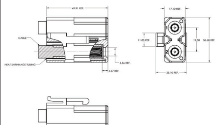
C10-752162-000 RADSOK® Plug, 5.7mm
