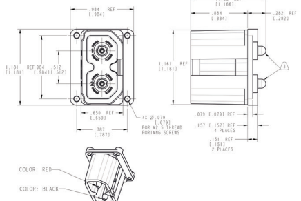
C10-752155-000 RADSOK® Receptacle, 3.6mm
