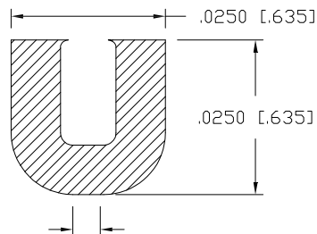
NOTE 1 CONTACT AREA SECTION C-C SCALE 40/1
