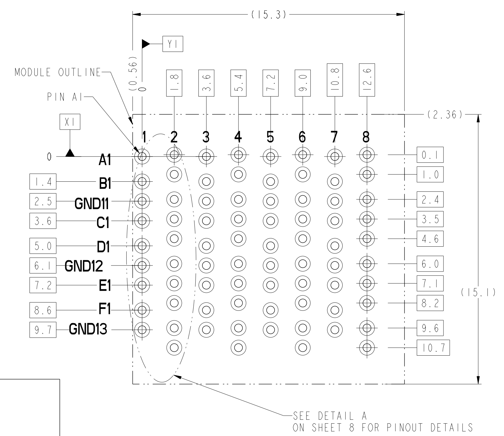
BP HOLE PATTERN COMPONENT SIDE RIGHT WALL MODULE BACKPLANE FOOTPRINT
