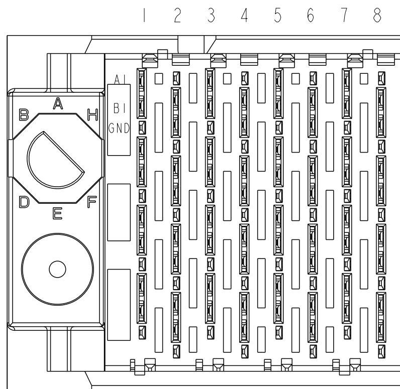
LEFT POLARIZING/GUIDE MODULE
