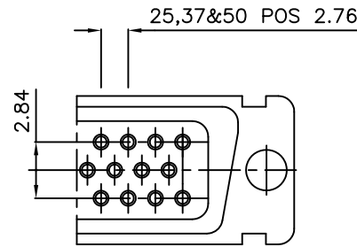
LAYOUT OF 50 POS.CONNCTOR
