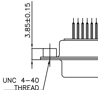
UNC 4-40 RIVETTING NUT
