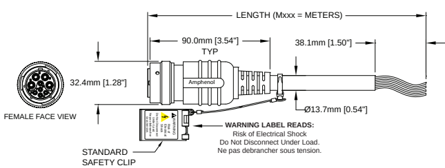
FIG 2: Female, Plug, Straight, 9 Position
