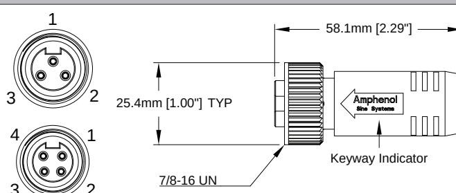
FIG 2: Female, Plug, Straight, Drop/Branch, 3 and 4 Position
