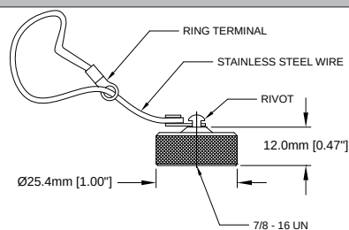
FIG 12: Male, Dustcap, Internal Threads
