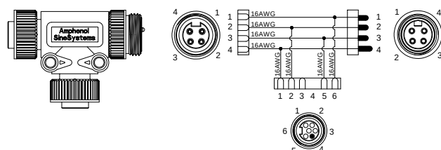
FIG 11: Shorting Plug, E-Stop Out, Red, 6P/5U
