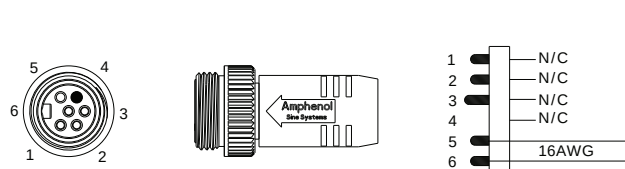
FIG 10: Shorting Plug, E-Stop In, Black, 6P/5U
