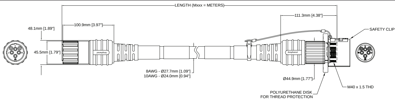
FIG 2: Male Plug to HAN Q4/2 Female Plug
