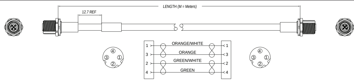
FIG 7: P29931-Mxxx, Ethernet M12, Female to Female, Receptacle, Orange
