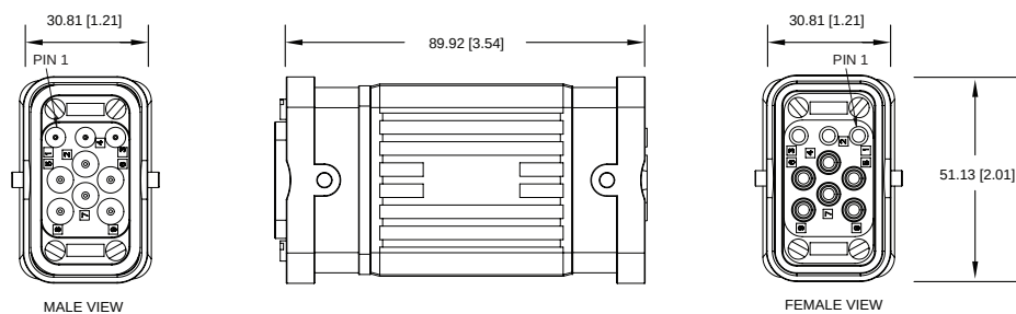
FIG 9: Male, 120V, Terminator, 9 Position
