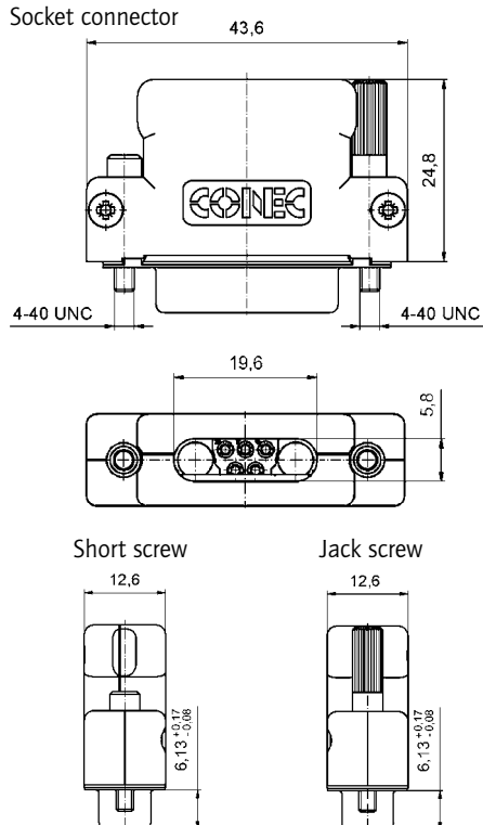
Socket connector
