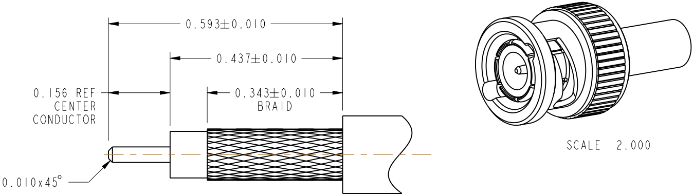
RECOMMENDED CABLE STRIPPING DIMENSIONS
