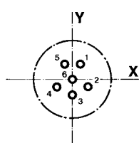
8-35 6 contacts Size 22D
