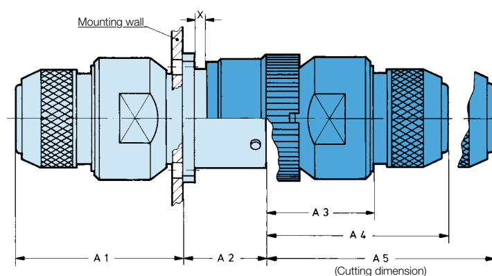
SJT 00 RT with backshell SQ
