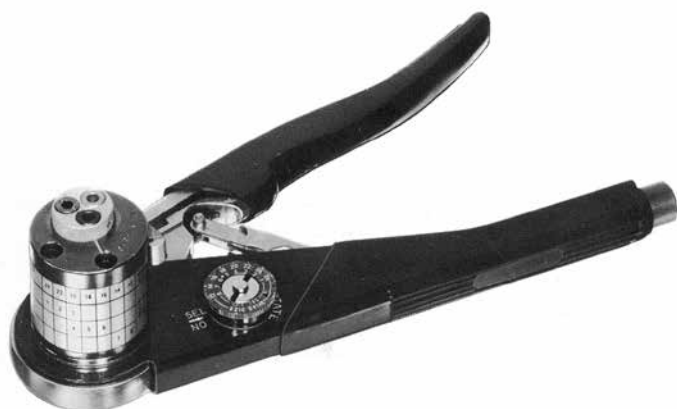
Crimp tool M 22520/1-01 (8-notch crimping)
