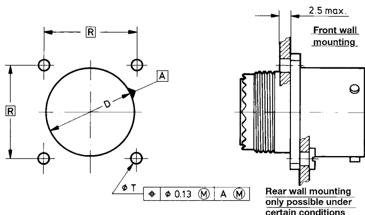
Mounting hole
