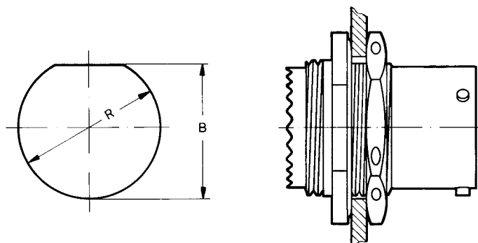
Mounting hole
