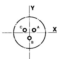
8-98 3 contacts Size 20
