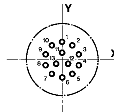
10-35 13 contacts Size 22D
