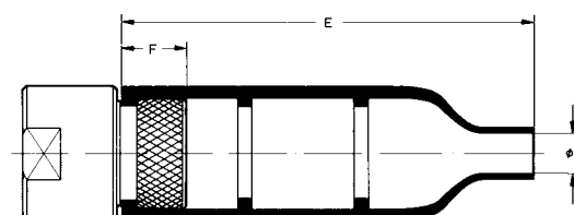
Backshell F with molded part 202
