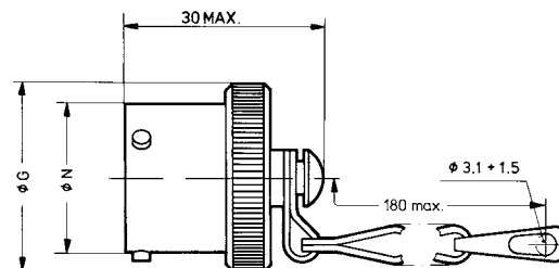
Metal protective cap (for design type 06) (VG 96912 V3XX)
