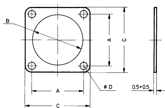
Flange gasket 10-101949 (VG 95328 T 0 7 A)
