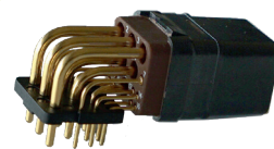
Female module with angled PCB contacts
