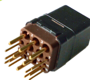
Female module with straight PCB contacts
