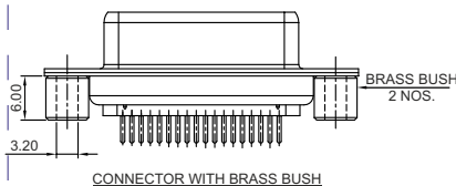
CONNECTOR WITH BRASS BUSH
