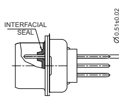
PLUG CONNECTOR WITH INTERFACIAL SEAL
