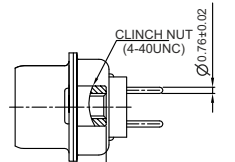
CONNECTOR WITH CLINCH NUT (4 - 40UNC THREAD)
