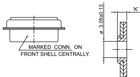
STD-THROUGH HOLE.
