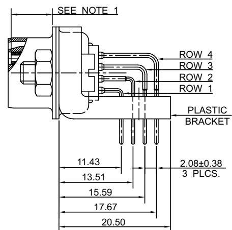
78 PIN (4 ROWS)
