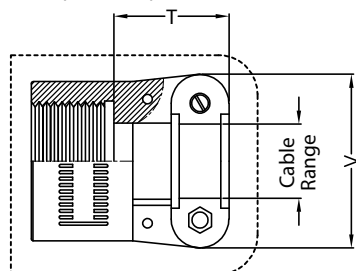
Style-H Clamp Heavy Duty (Table-2)
