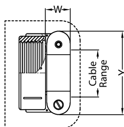
Style-S Clamp Medium Duty (Table-3)
