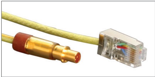
Quadrax Pin with 8P8C "RJ45" Jack
