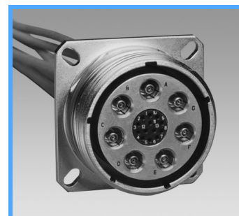
Ground Plane Connector with Metallic Insert and Concentric Twinax Contacts
