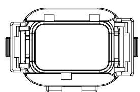
KEY-D CONFIGURATION P/N ATM06-08SD-CAP INSERT COLOR: BROWN
