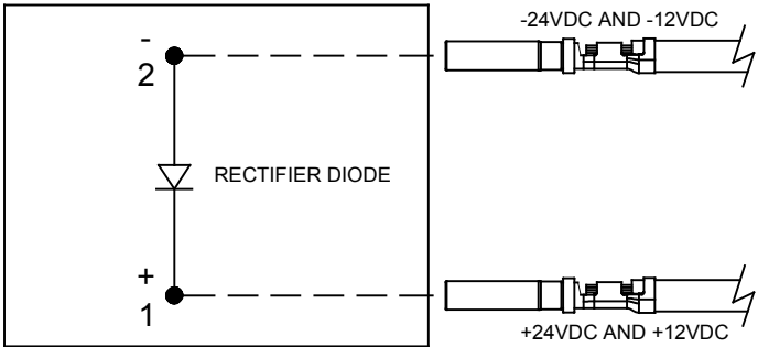
CONNECTOR DIAGRAM
