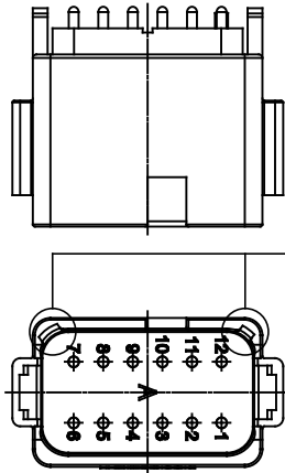
P/N AT04-12PA-BMXX KEY-A CONFIGURATION COLOR: GREY
