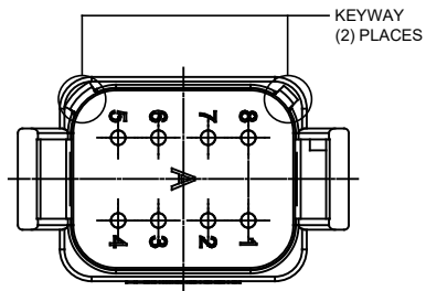
P/N AT04-08PA-BMXX KEY-A CONFIGURATION COLOR: GREY
