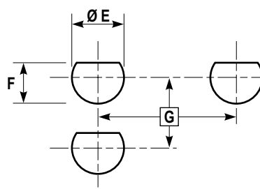
Jam nut receptacle rear panel mounting
