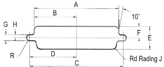
Standard cutout
