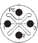
Male connector 3-pos.+PE
