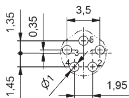
Male connector 5-pos. B-coded
