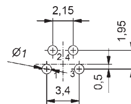
Male connector 4-pos.
