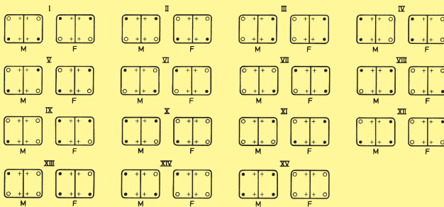
Figure 3: Connector with two mounting frames
