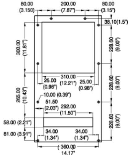
Drilling Template
