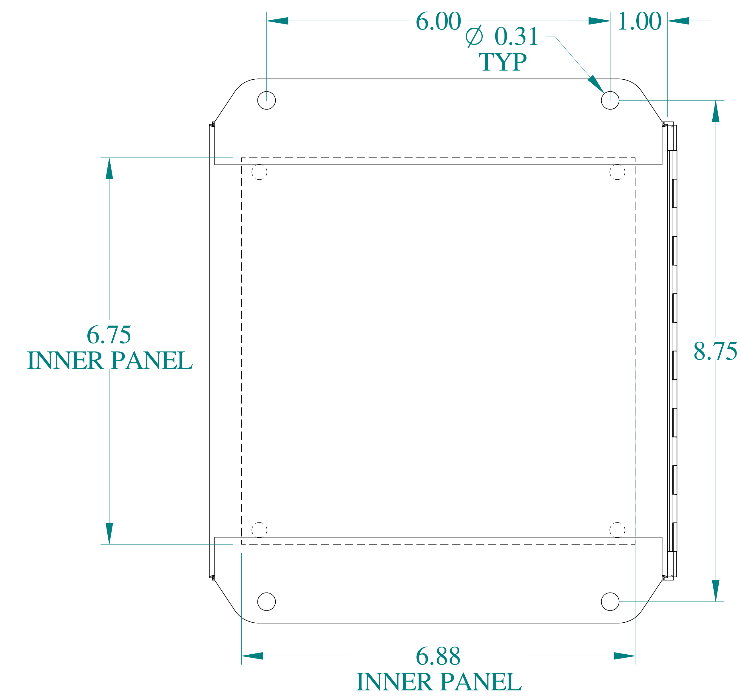
BACK VIEW
