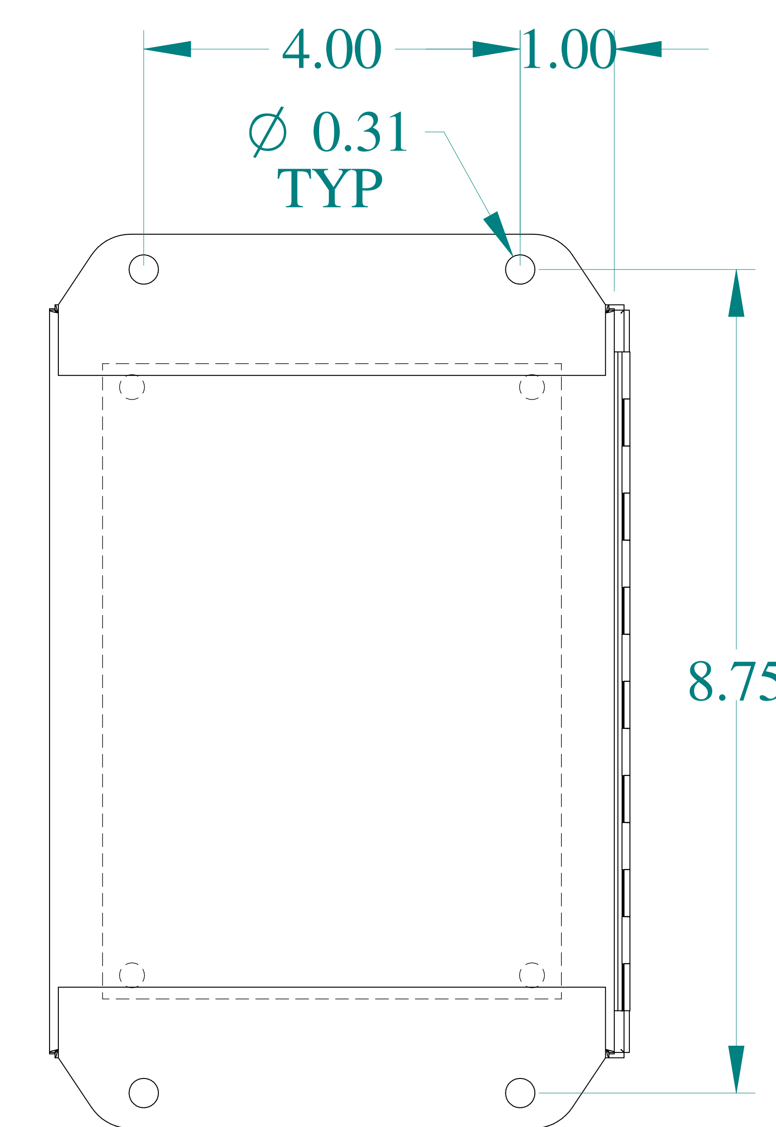
BACK VIEW
