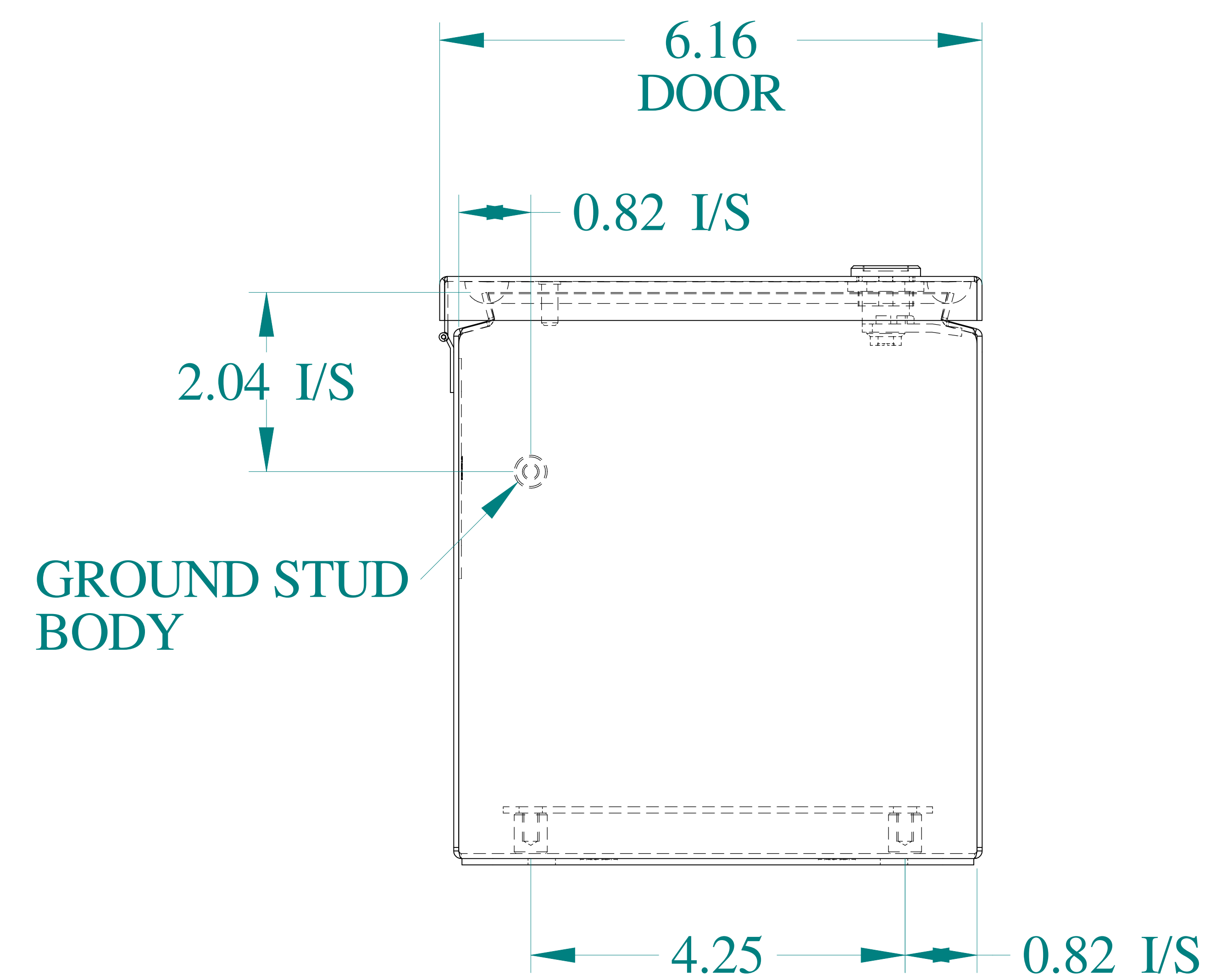
BOTTOM VIEW
