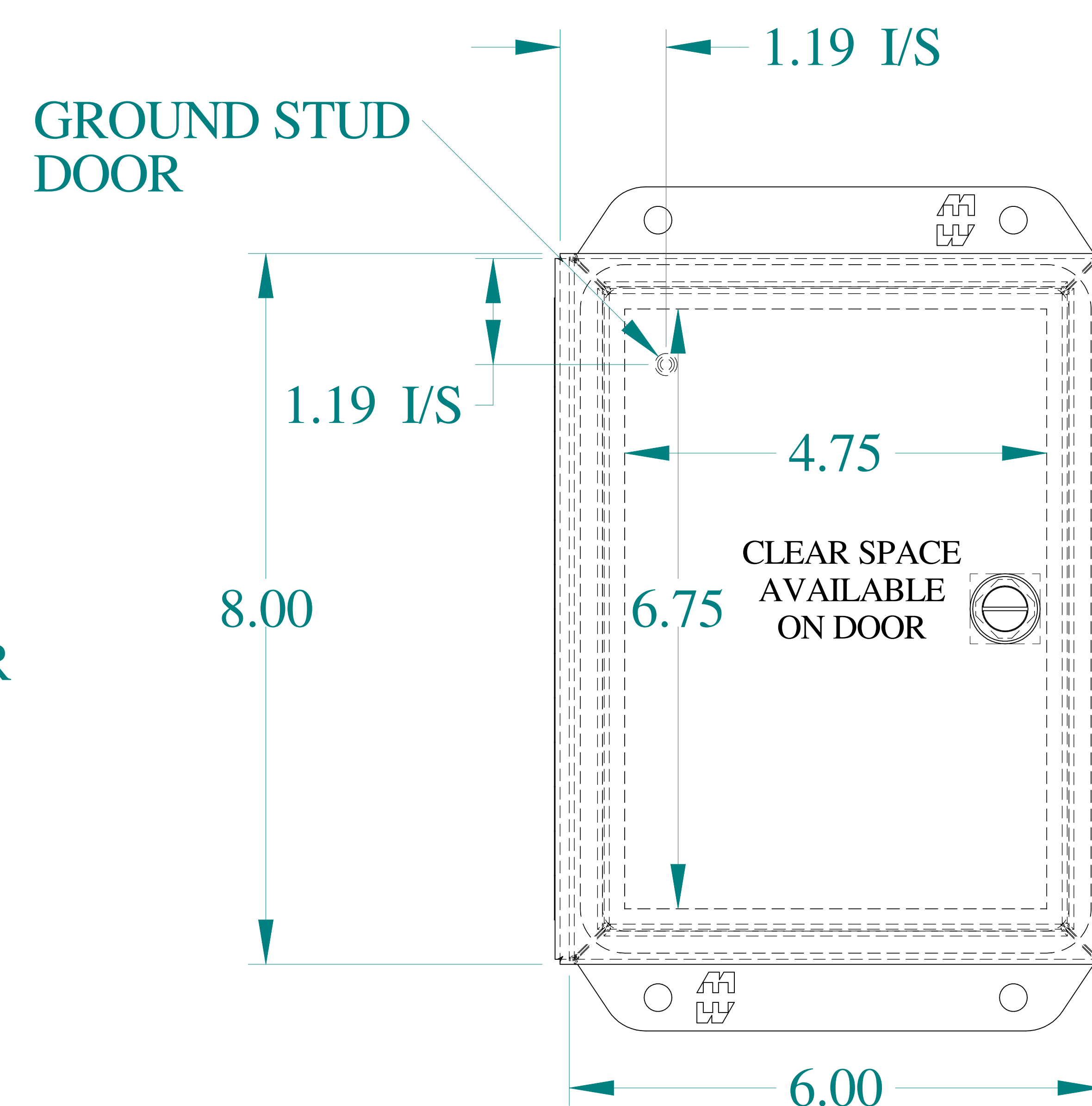
FRONT VIEW
