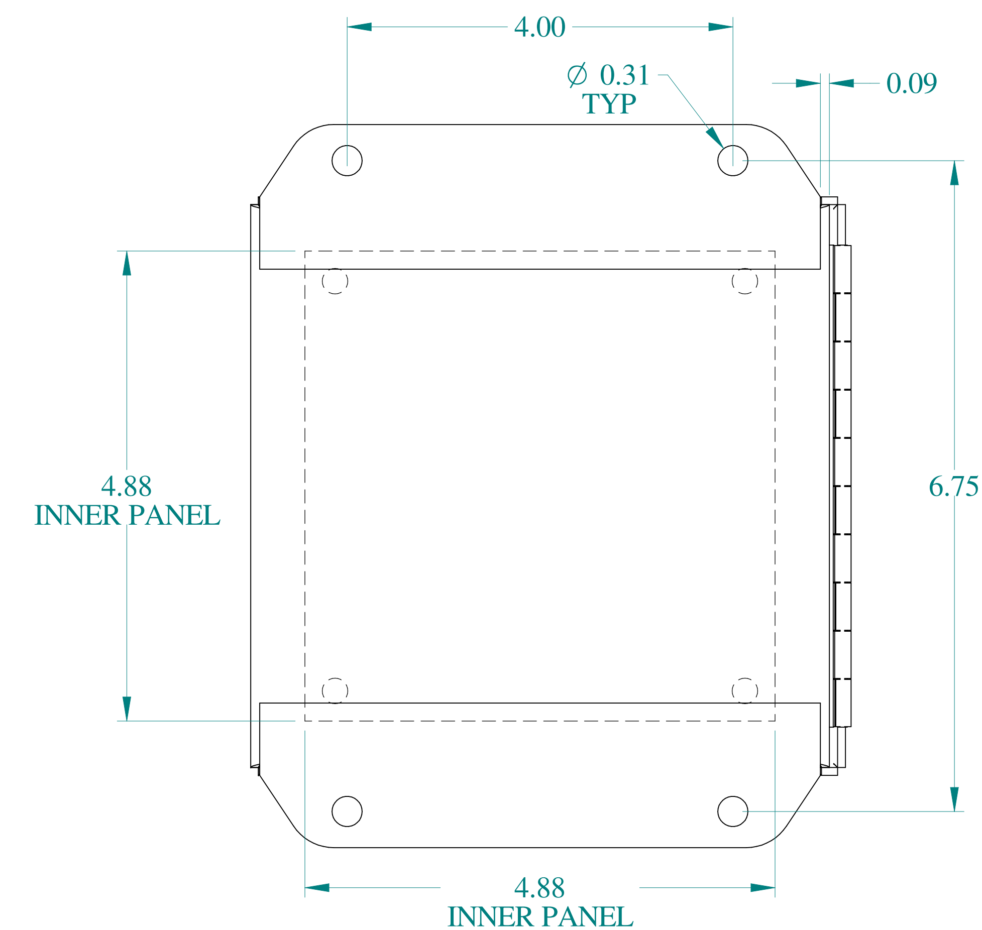
BACK VIEW
