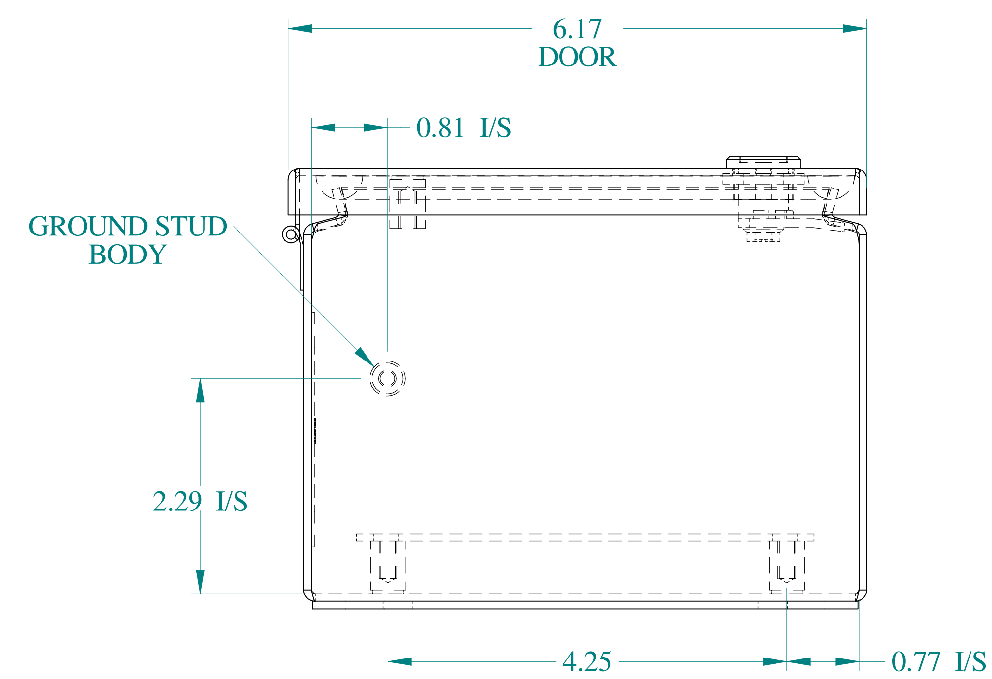
BOTTOM VIEW
