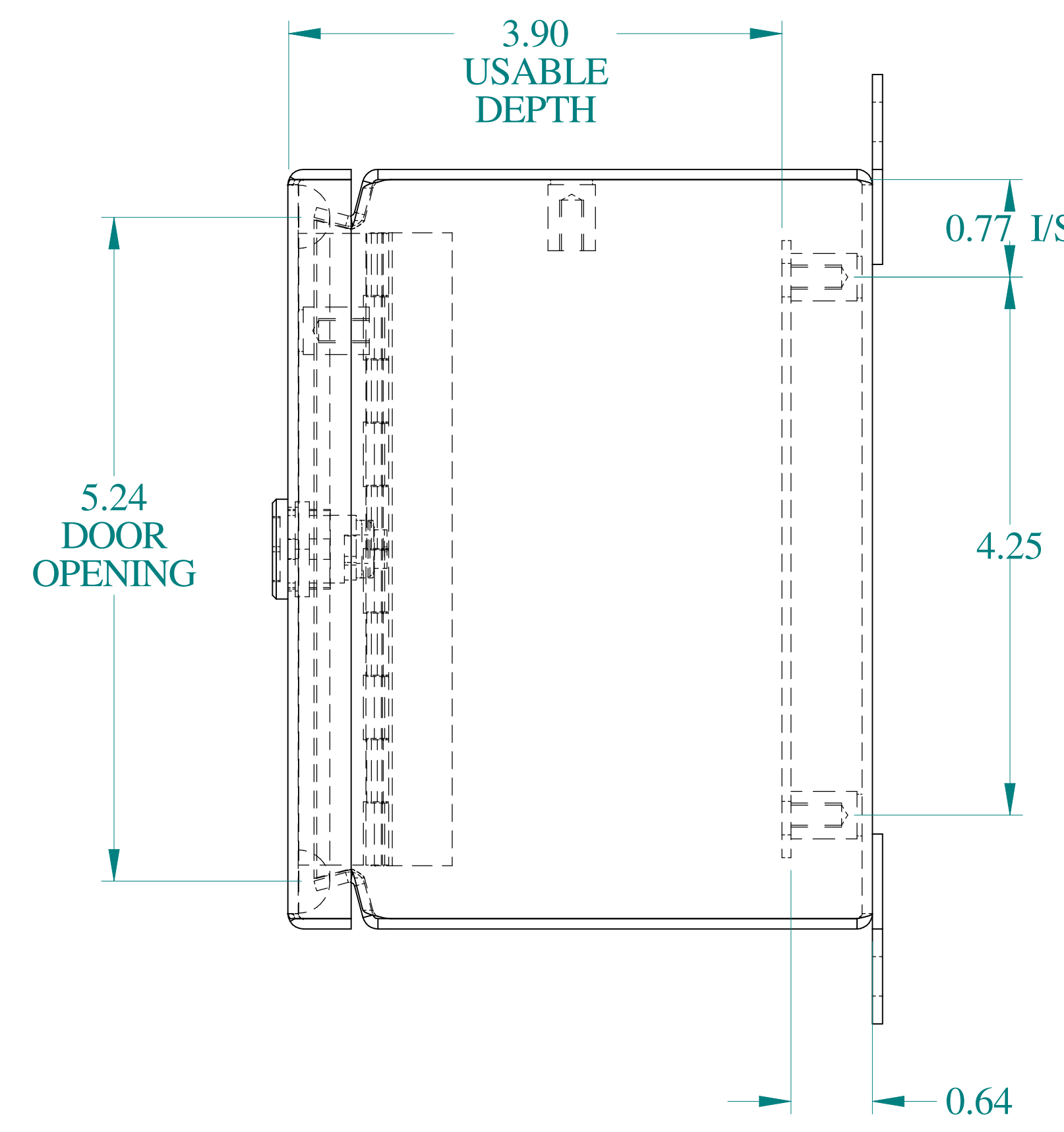
SIDE VIEW
