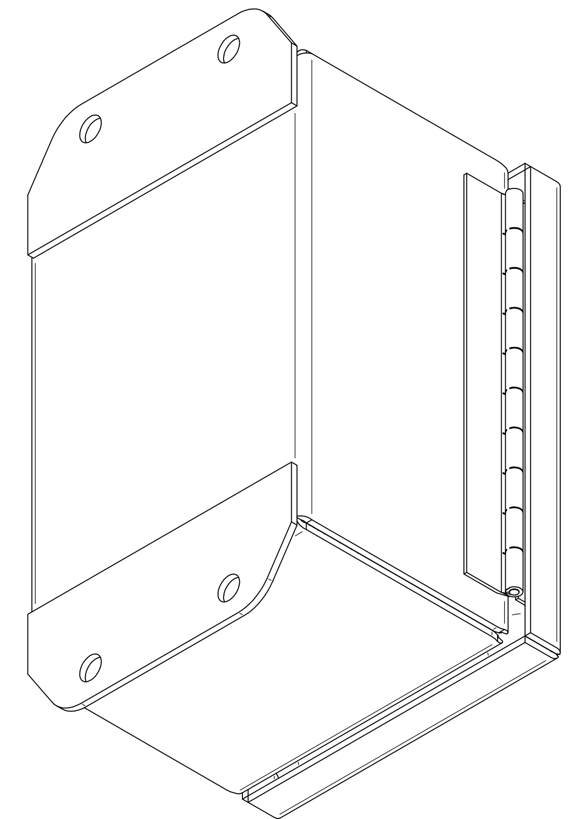
ISOMETRIC VIEWS
