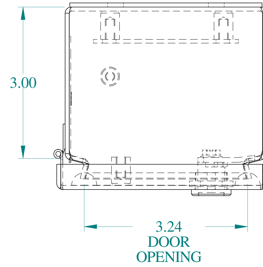
TOP VIEW
