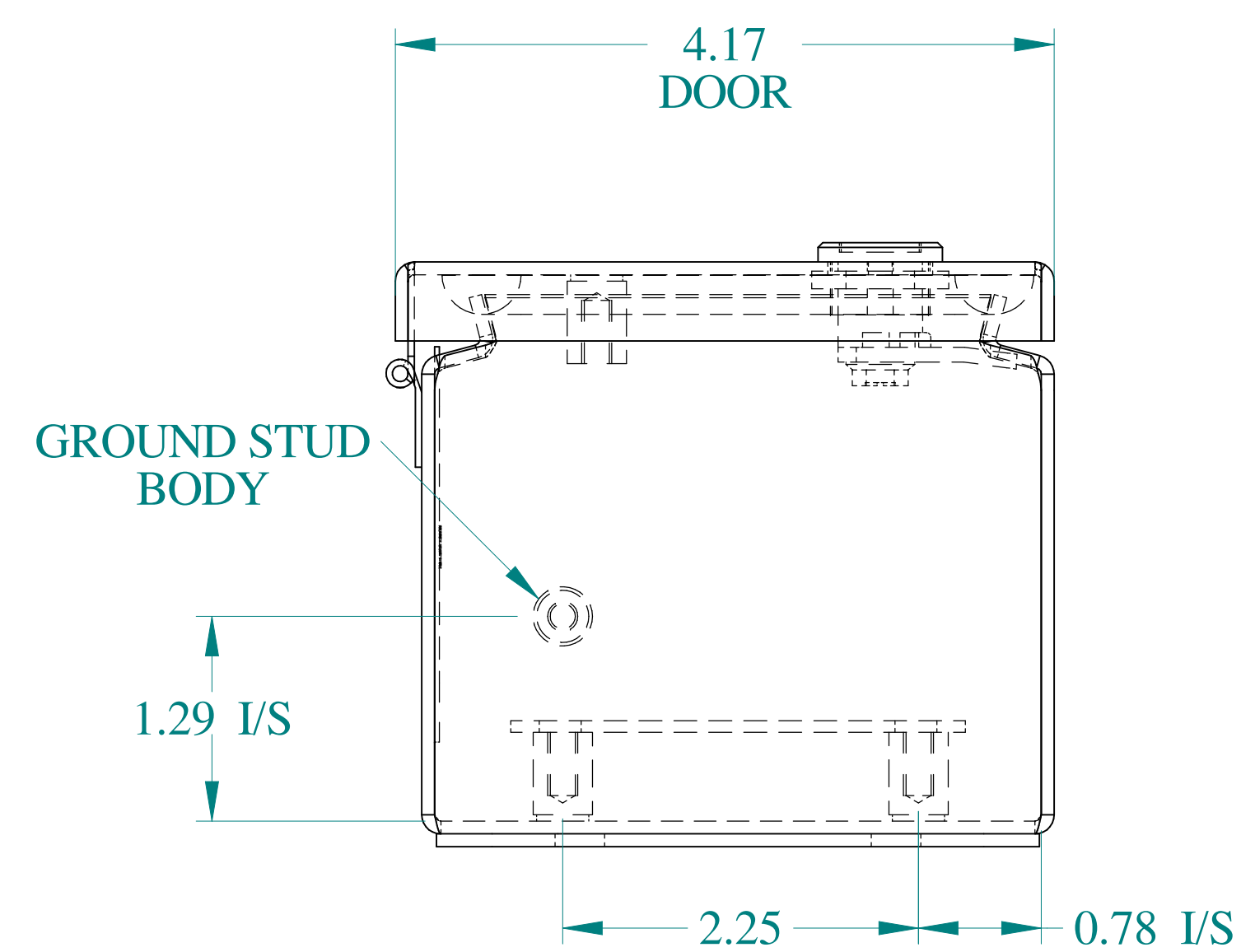
BOTTOM VIEW
