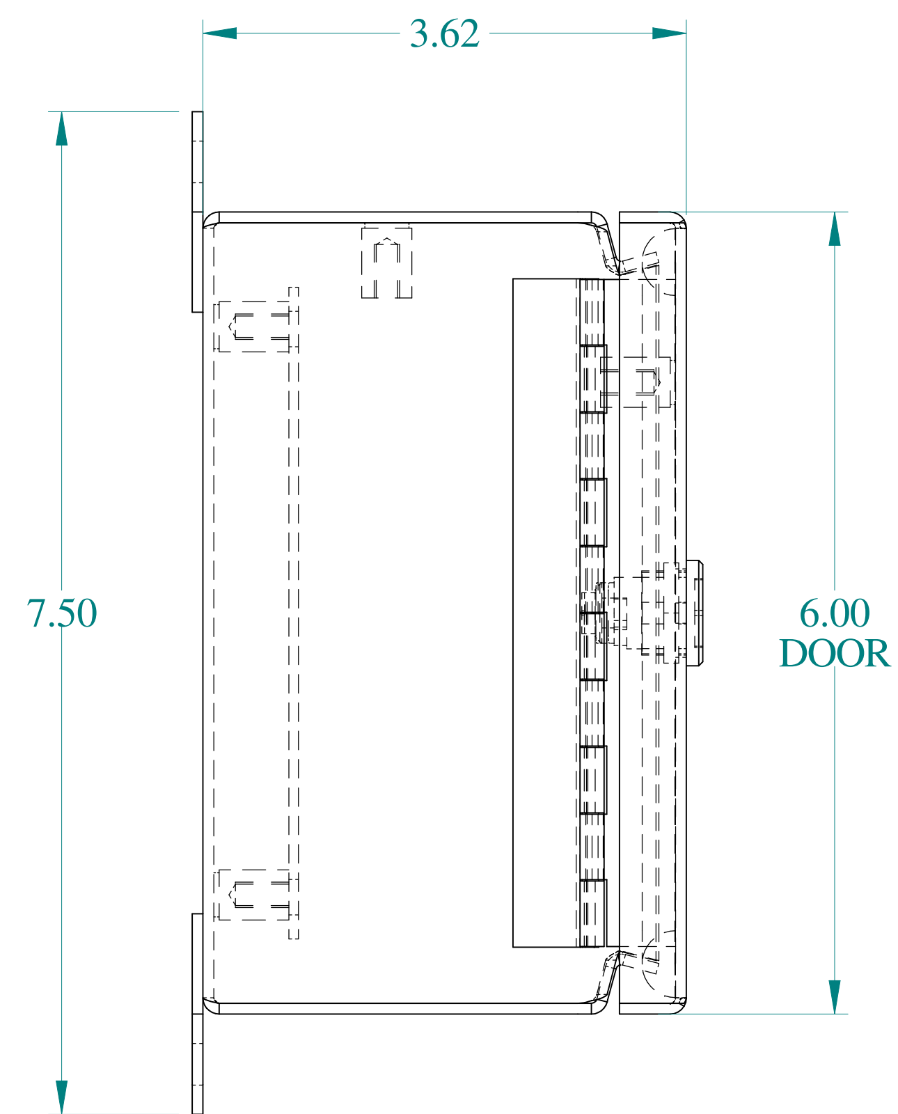
SIDE VIEW
