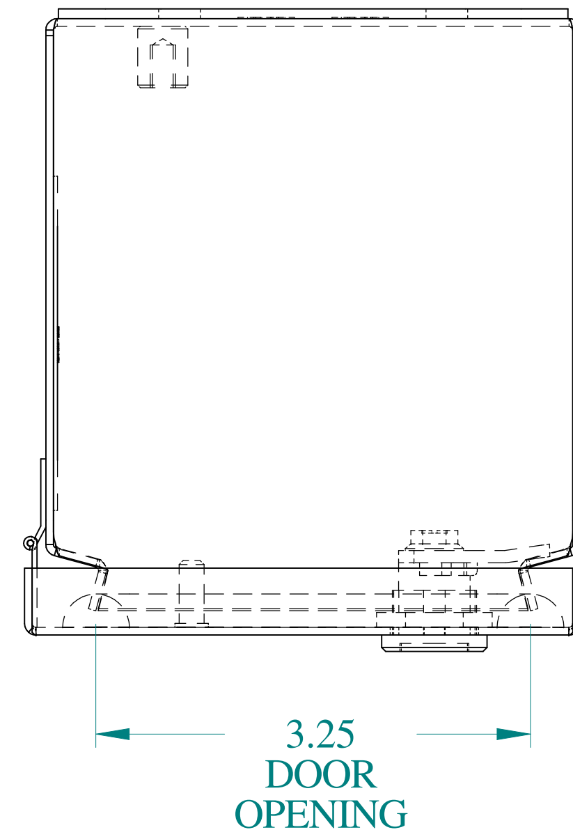
TOP VIEW
