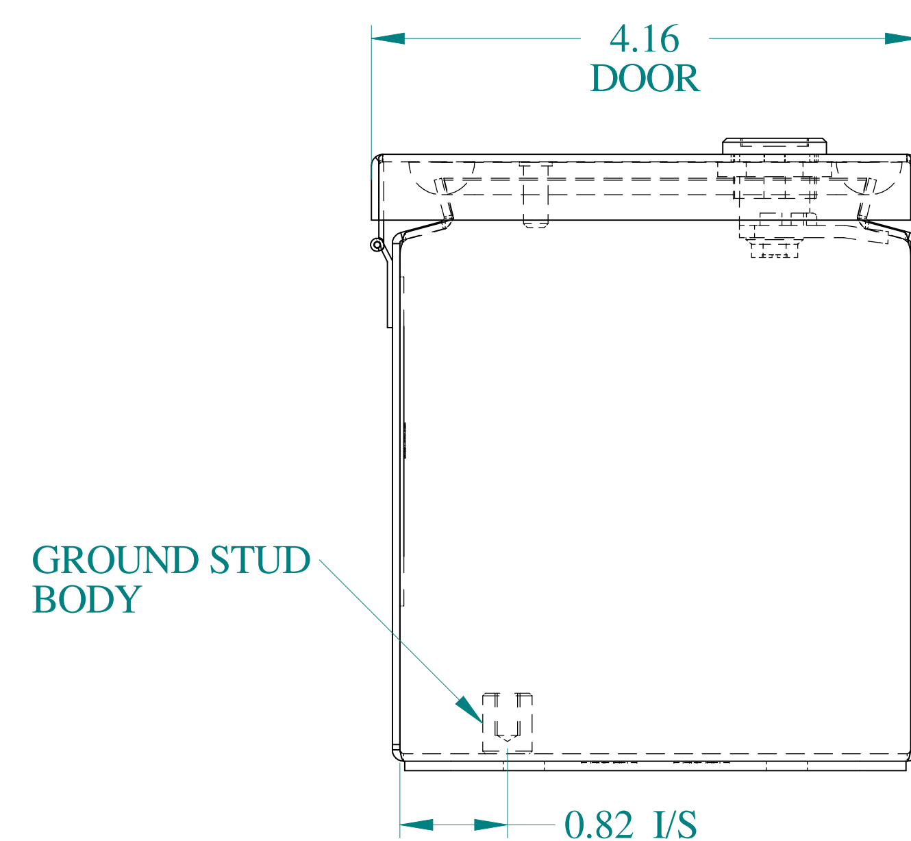
BOTTOM VIEW
