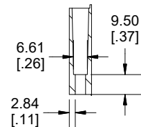
SECTION C-C MOUNTING HOLE
