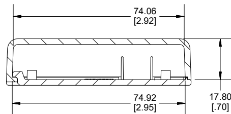
SECTION B-B END VIEW
