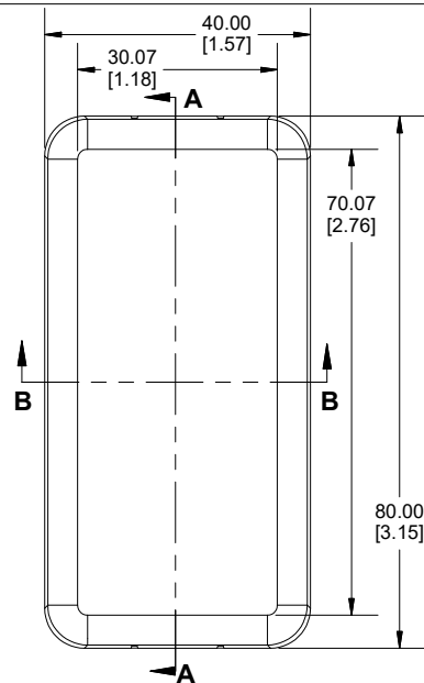
TOP VIEW
