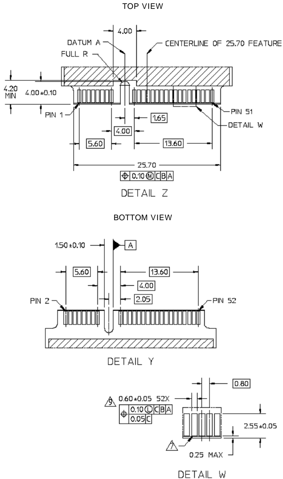
Figure 3-2: mSATA ArmourDrive Connector
