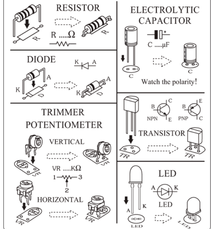
Figure 1 Installing components
