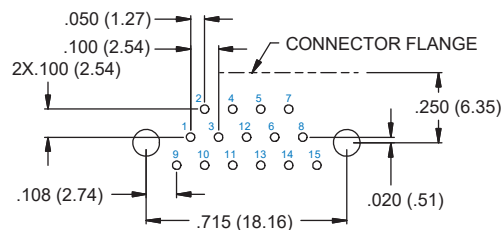
15 PIN
