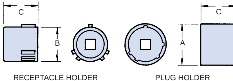
RECEPTACLE HOLDER
