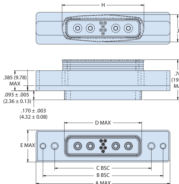
SHELL SIZES H & L H-10P4 SHOWN
