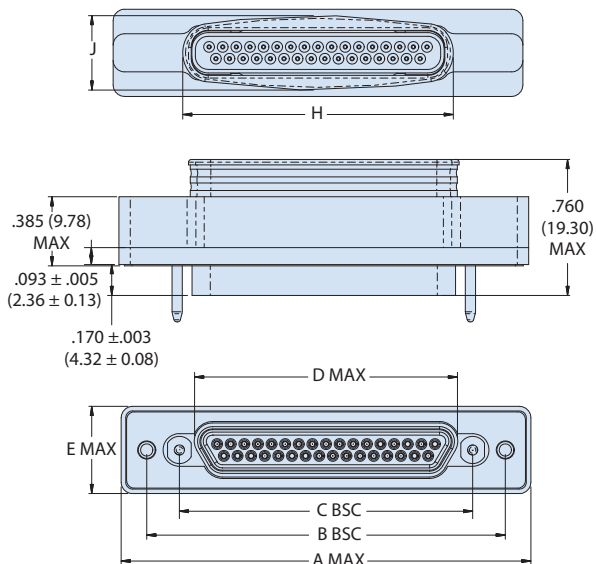
SHELL SIZES A THRU G, J, & K J-33 SHOWN (NOTE THAT SIZE G HAS 3 CONTACT ROWS)
