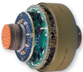
EMP Diode-Equipped Connector with Oversized Shell
