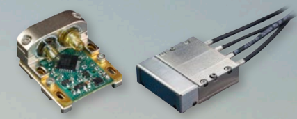
PCB-Mount Opto-Electronic Transceivers
