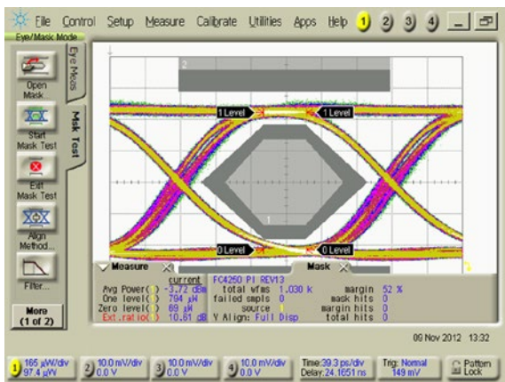
4.25 Gbps / +25°C
