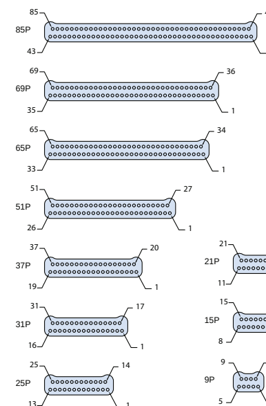
D-Subminiature Connector 25 Contacts on 0.109 Inch Spacing
