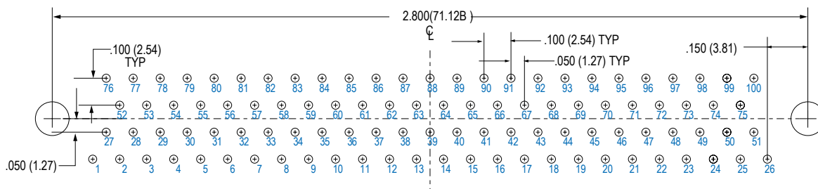
100 SOCKET M83513/27-H
