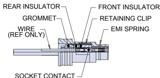
CROSS-SECTIONAL VIEW OF 790-046S
