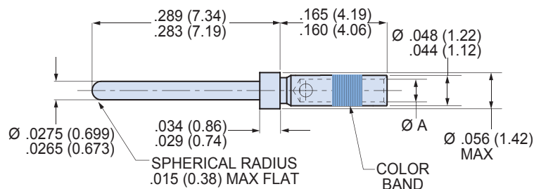
#23 Pin Contact
