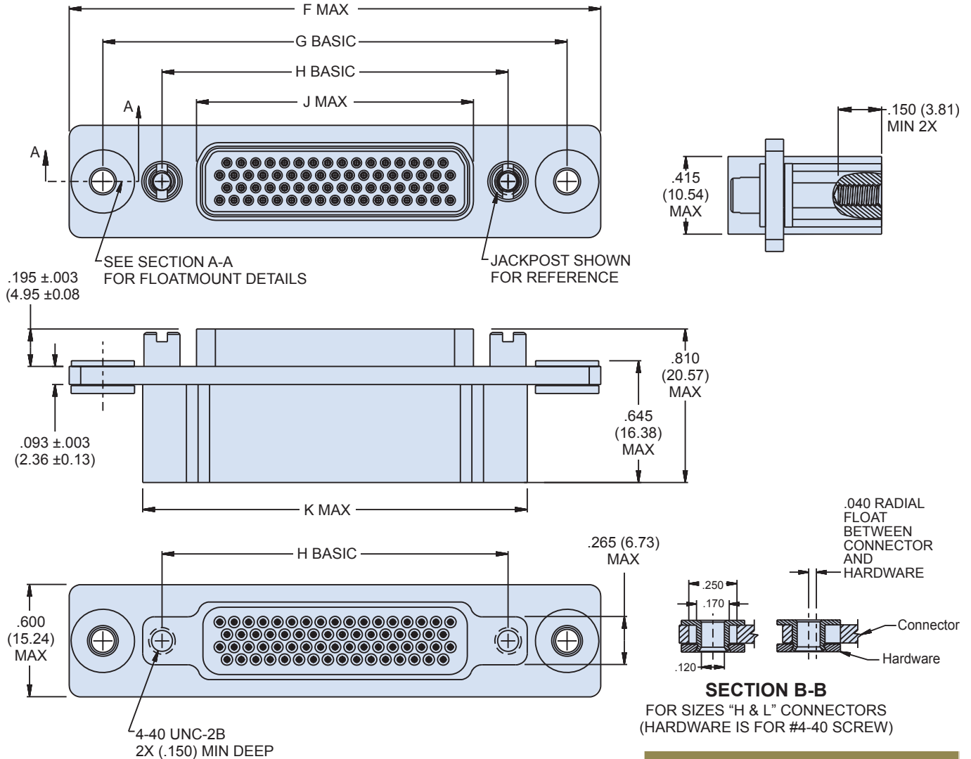
790-050P SIZES H & L DIMENSIONS
