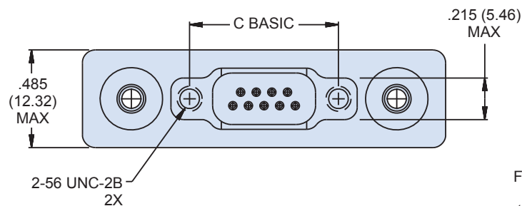
790-050P SIZES A, B, C, D, E, F, G, J & K DIMENSIONS
