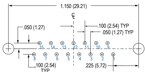
15 PIN
