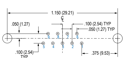
9 PIN
