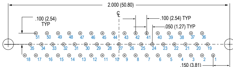
51 PIN
