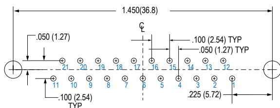
21 PIN
