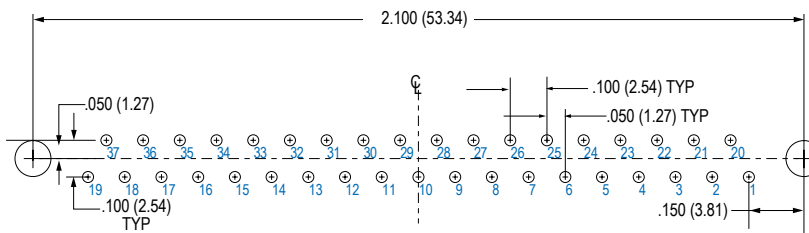
37 PIN
