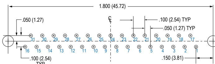
31 PIN
