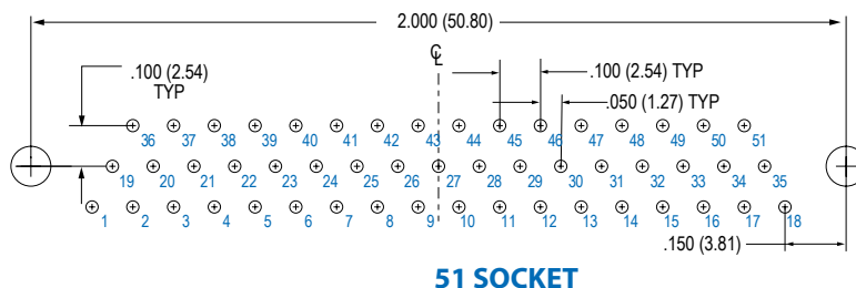
51 SOCKET
