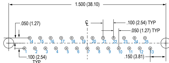
25 SOCKET
