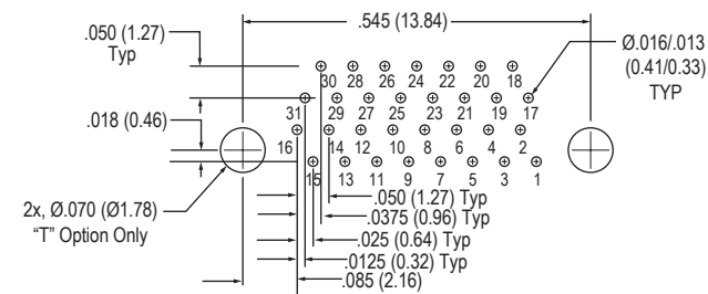
31 Contacts
