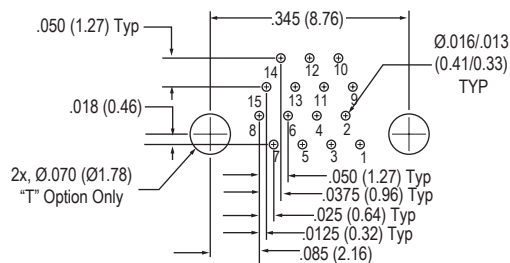
15 Contacts
