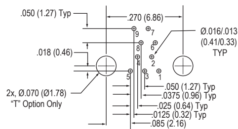
9 Contacts
