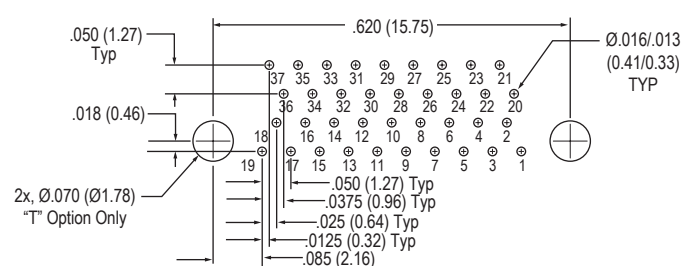
37 Contacts
