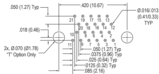
21 Contacts
