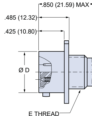
Accessory Thread 803-004-02
