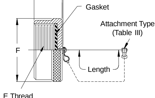
660-011 Receptacle Cover
