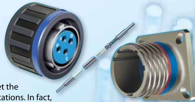
Glenair MIL-DTL-38999 Series III Type fiber optic connectors and MIL-PRF-29504 qualified termini for use in Mil-Aero applications.
