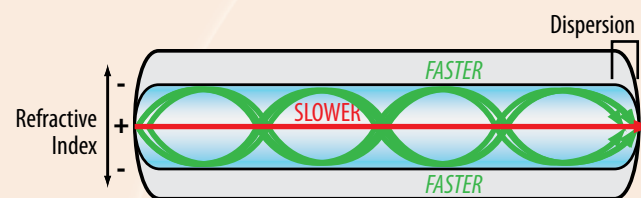
Graded-Index Multimode fiber's core has a refractive index that decreases from the center to the edge. Light rays moving down the center axis move slower than those at the edge, which take a curved path instead of zigzagging as they do in step-index fiber. The modes at the edges arrive closer together with the modes in the middle which allows for less dispersion in the pulse.
