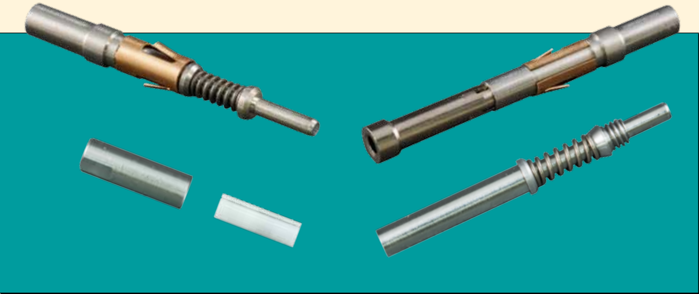
Factory terminated lens pin contact (top) and lens socket contacts on pigtail wires allow for easier fusion splicing in the field.
