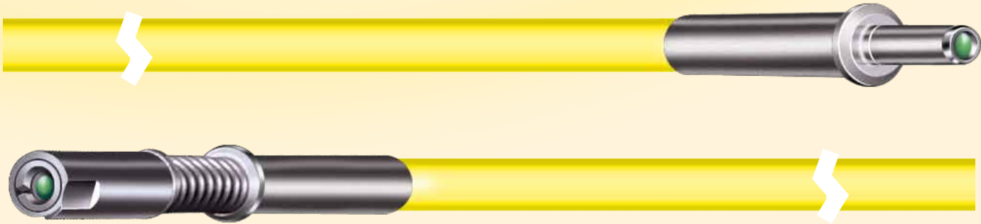
Factory terminated lens pin contact (top) and lens socket contacts on pigtail wires allow for easier fusion splicing in the field.
